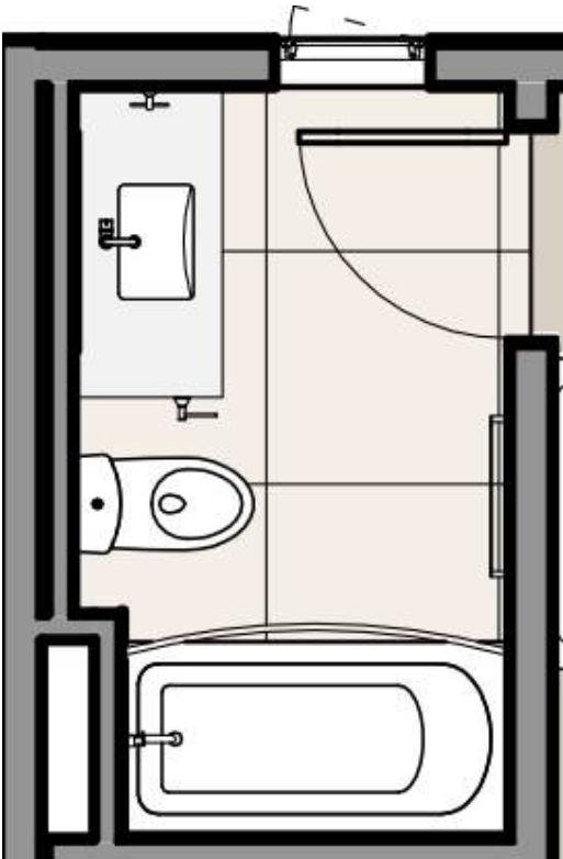
GUEST BATHROOM 2 ENLARGED PLAN scale= 3/8" - 1'0"
